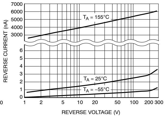
Figure 3. Reverse Leakage
